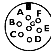
Connector view
