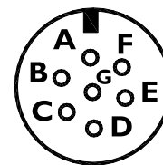
Connector view
