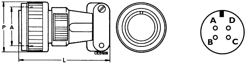
Connector view
